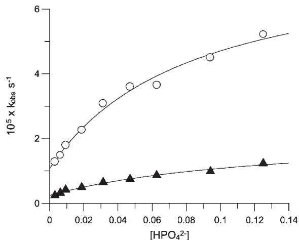
Figure 1. Dependence of the observed first-order rate coefficient on buffer concentration for MHBnT (○) and MHBnT-C2 \alpha -d (▲) at 40 °C, I = 1.0 . Curves are fitted to the Keefe–Jencks equation for a mechanism with a buffer-dependent change in rate-determining step
