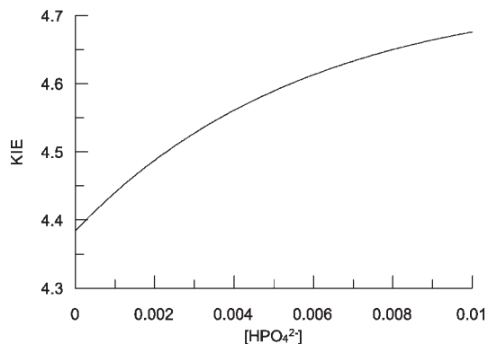
Figure 2. Observed KIE on fragmentation as a function of hydrogen phosphate buffer concentration
